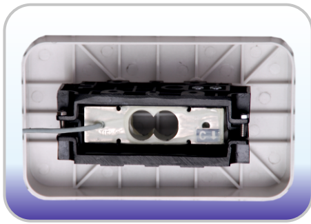
Ip65 loadcell with special environment protection
